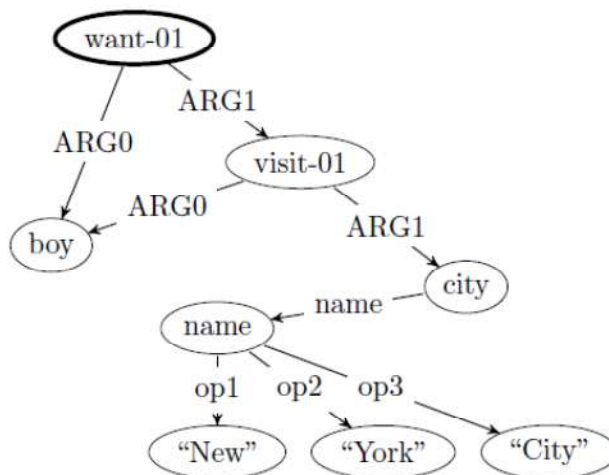
Figure 9: a graph of an AMR sentence (Flanigan et al.). The head want has two arguments: boy and visit . Here both arguments have different duplicate roles: the object, visit , also functions as a head node for its own arguments while boy functions as a subject for both want and visit , as denoted with arrows pointing from these verbs towards the subject (ARG0).
