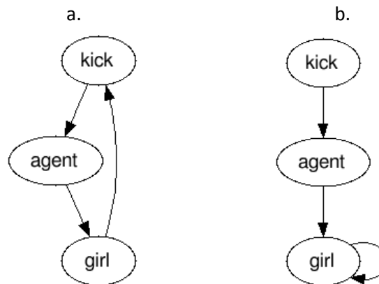
Figure 16: (a.) an FG1 sentence as the DOT command kick->agent->girl->kick , and (b.) another FG1 sentence as the command kick->agent->girl->girl generate cyclic graphs. This is in excess of the expressive power of all PSGs.
