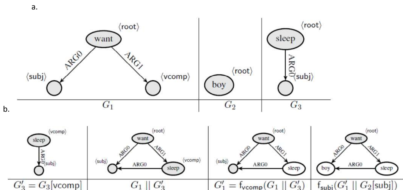
Figure 10: (a.) three s-graphs representing the sentence "the boy wants to sleep"; (b.) these are combined into a common graph using a mathematical method (from Koller 2015).
