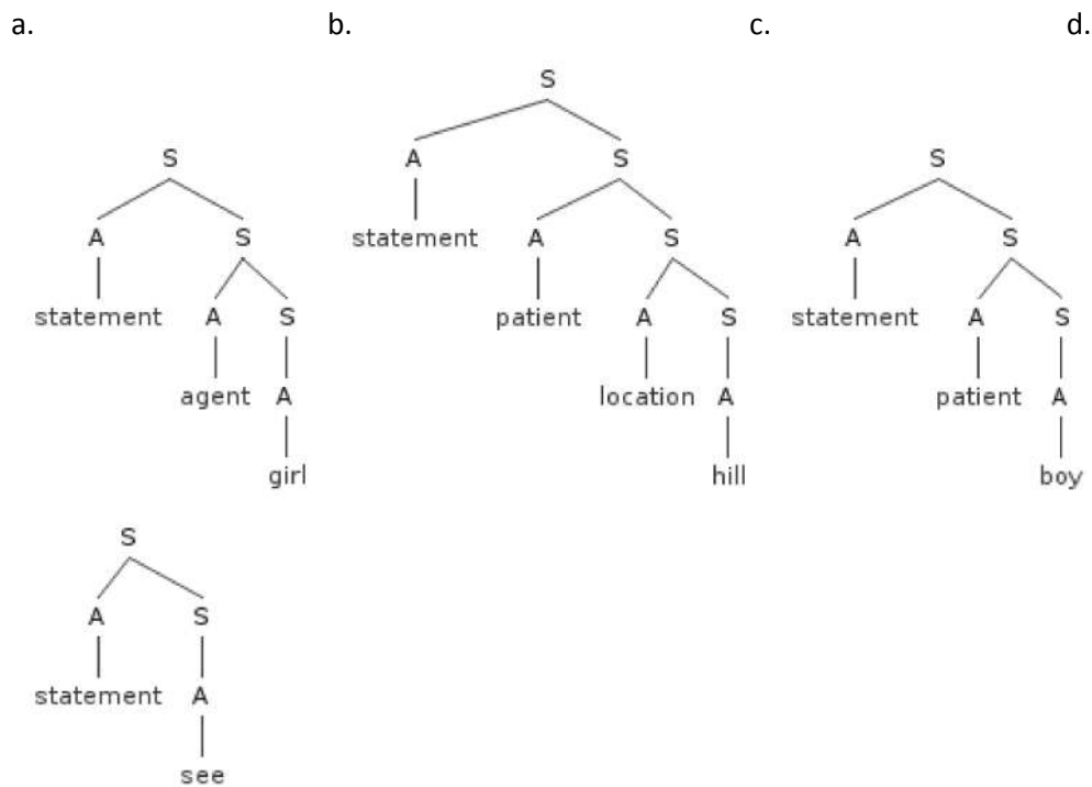
Figure 8: the four branches of an FG2 sentence (cf. figure 7) converted into the regular grammar S \rightarrow AS \mid A (with right to left input), analysed by a CYK parser, generates four trees with the total of 36 symbols.
