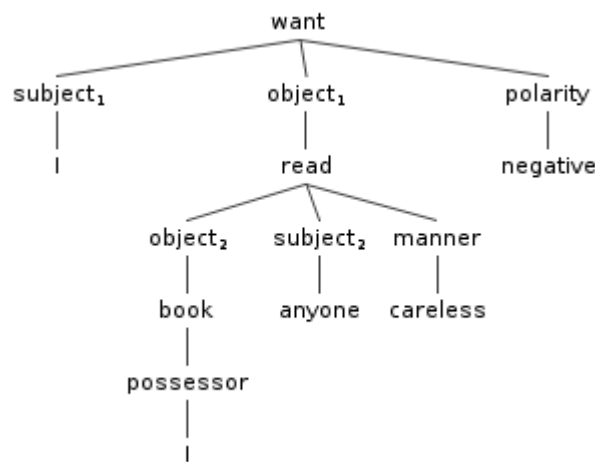
Figure 13: the example sentence in a dependency tree. Instead of including labelled edges, all values have their own node in the tree. Dependencies are expressed as nondirected lines, assuming a top-down direction. Here joining of the two same-identity instances of I does not occur.
