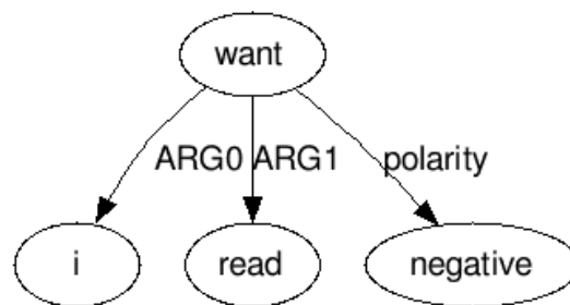
Figure 11: a directed tree for the ABAS phrases "want ARG0 i", "want ARG1 read" and "want polarity negative".
