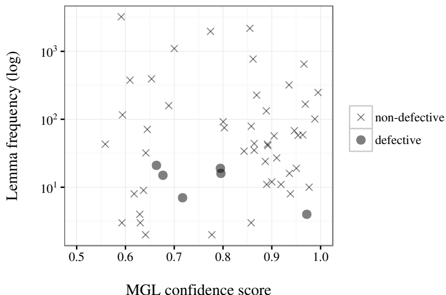
Figure 1: Confidence scores and frequencies of Spanish third-conjugation mid vowel stem verbs.
