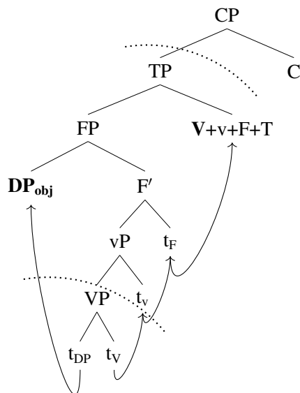
(6) V-raising grammar
