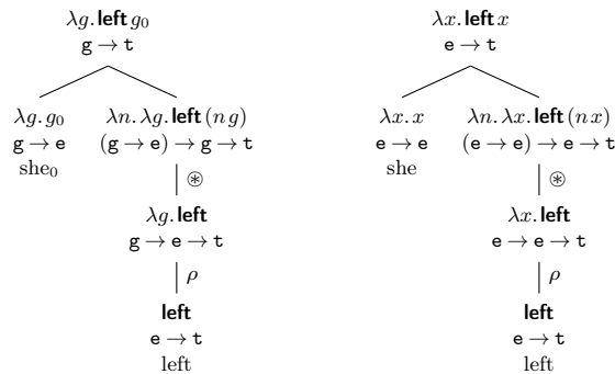
Fig. 8. Variable-full (left) and variable-free derivations (right), applicative-style.
