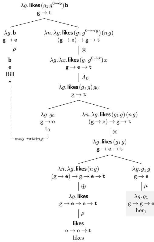
Fig. 6. Deriving a paycheck reading with a higher-order instantiation of the pronoun and a corresponding application of the monadic \mu . Given a \mathbf{g} such that \mathbf{g}_1 = \lambda g.\mathbf{mom} g_0 (i.e., the intension of his 0 mom ), the extension of this sentence at \mathbf{g} is likes (mom b) b .
