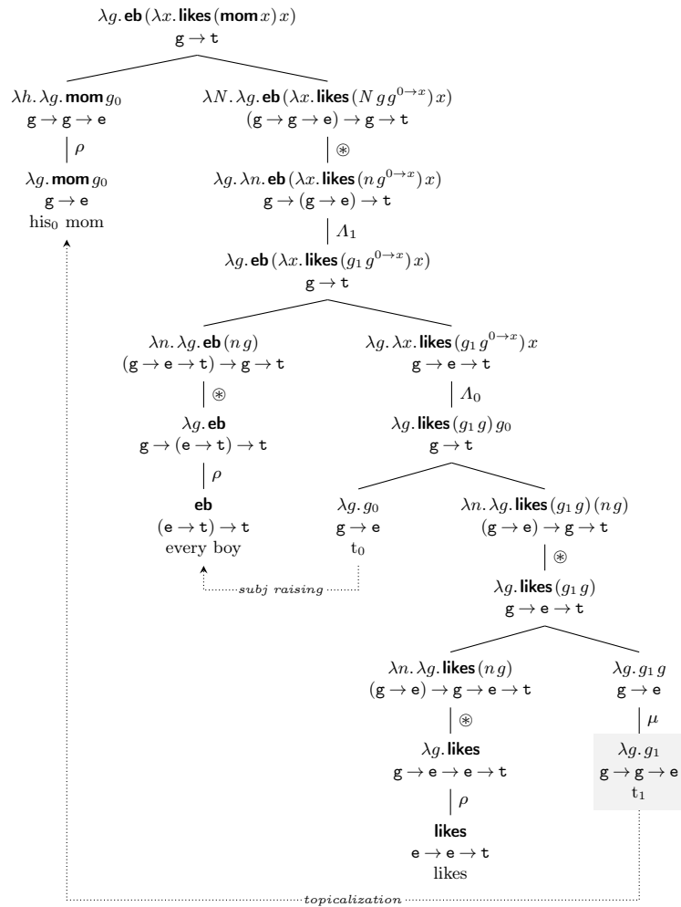
Fig. 7. Deriving binding reconstruction with a higher-order trace and a corresponding application of \mu . In contrast with the paycheck derivation, here the higher-order variable is resolved to an intra-sentential antecedent, via in-scope binding (precipitated by A_1 ).
