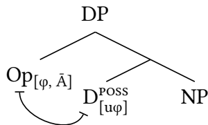
(293) Probe on D_{\text{POSS}} interacts with [\varphi] and [\bar{A}] on Op
